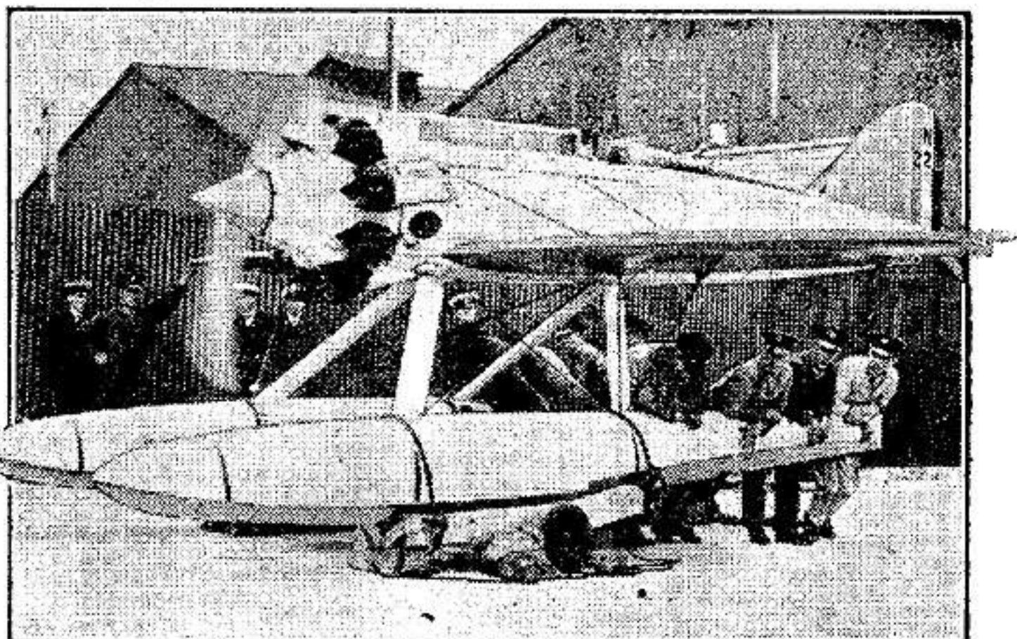
Will this monster of the air, named the “Crusader,” be the means of bringing back to Britain the coveted trophy known as the Schneider Cup? In the photo above is shown the Bristow-Short-Bristol “Crusader” with engine running. Note how many men are required on the streamlined floats to prevent the ‘plane from turning turtle while the engine is being raced.
