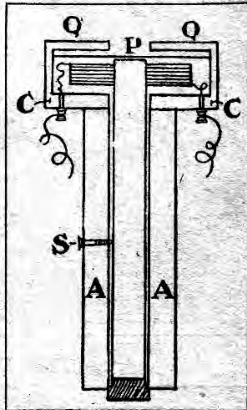
Fig. 3.—Section of the Complete Instrument.
