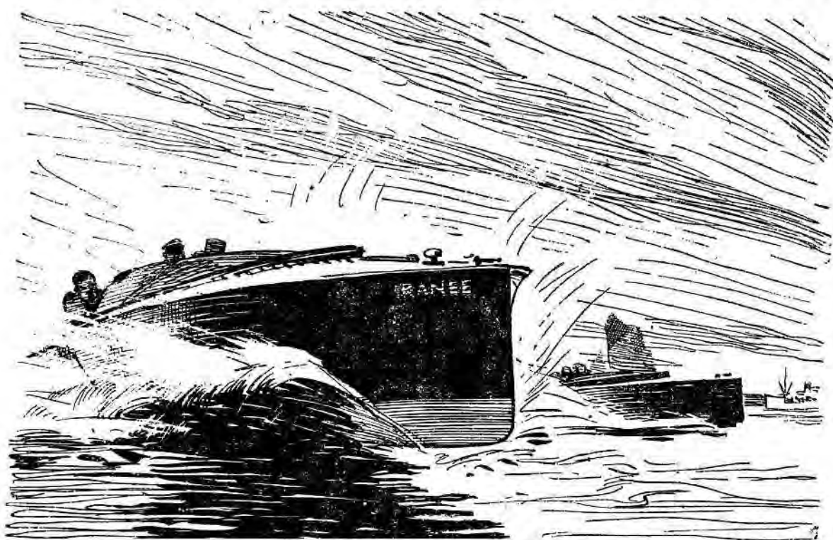
Out into the open Thames the Westward and the Rancee swept, cutting through the water like torpedoes and sending up a spray ten feet in the air.
